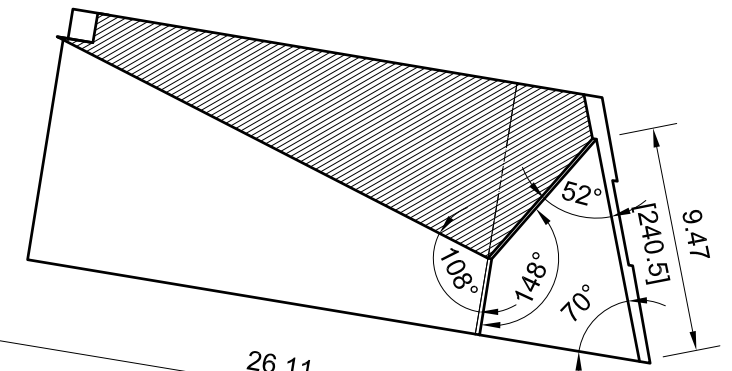
SECTION VIEW D7-36
