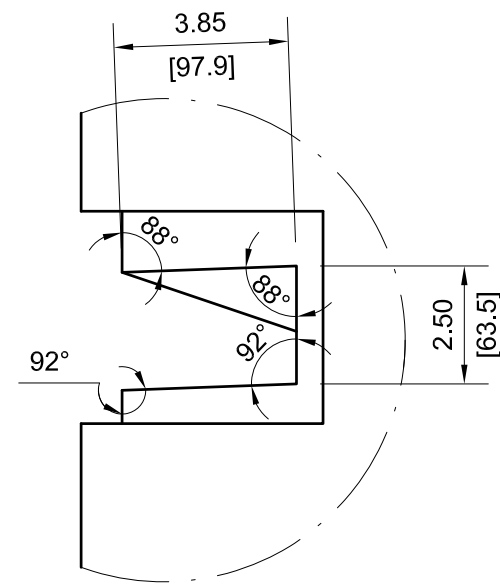
DETAIL VIEW E1-37
