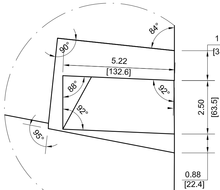
DETAIL VIEW C8-37
