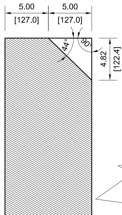
SECTION VIEW B6-47
