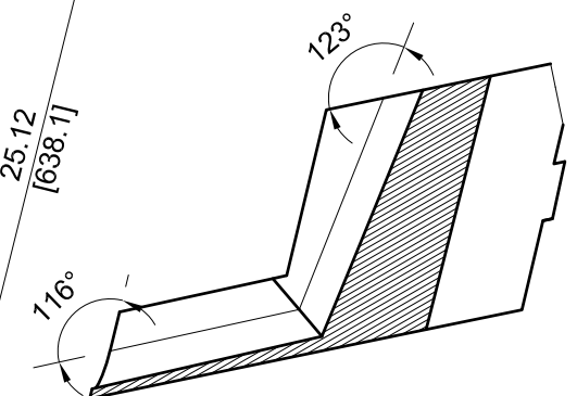
SECTION VIEW F6-27
