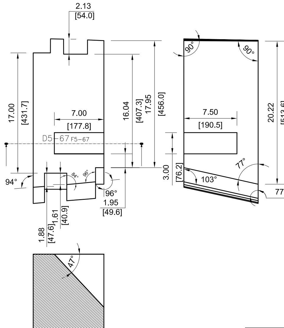
SECTION VIEW D5-67
