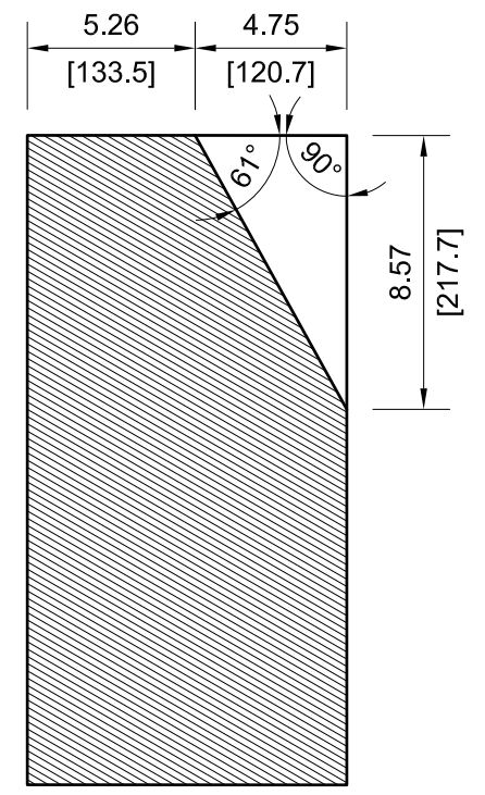
SECTION VIEW B6-46
