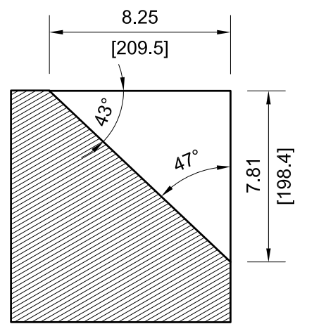
SECTION VIEW D6-43
