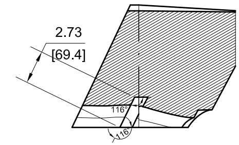
SECTION VIEW D4-25
