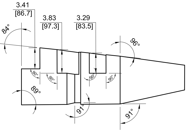
SECTION VIEW 1C5-169
