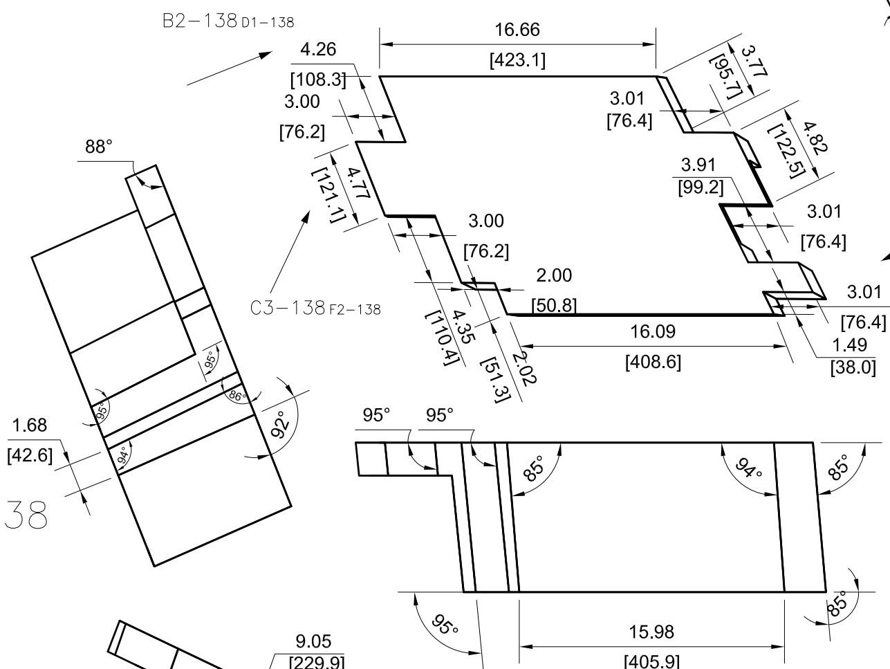
REAR VIEW RELATIVE TO VIEW C4-138
