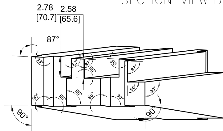
VIEW D4-187 REPEATED FOR CLARITY PURPOSES.
