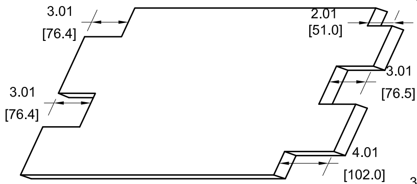
REAR VIEW RELATIVE TO VIEW D4-156
