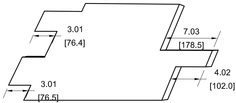
REAR VIEW RELATIVE TO VIEW D4-145
