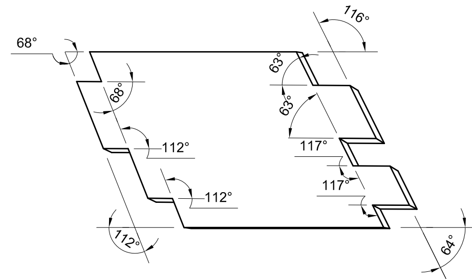
VIEW C4-140 REPEATED FOR CLARITY PURPOSES.
