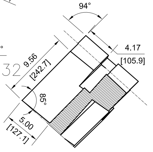
SECTION VIEW C4-132
