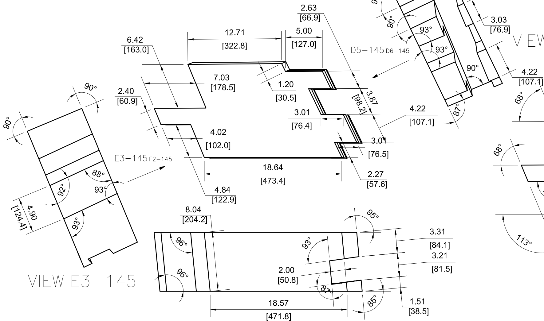
REAR VIEW RELATIVE TO VIEW D4-145
