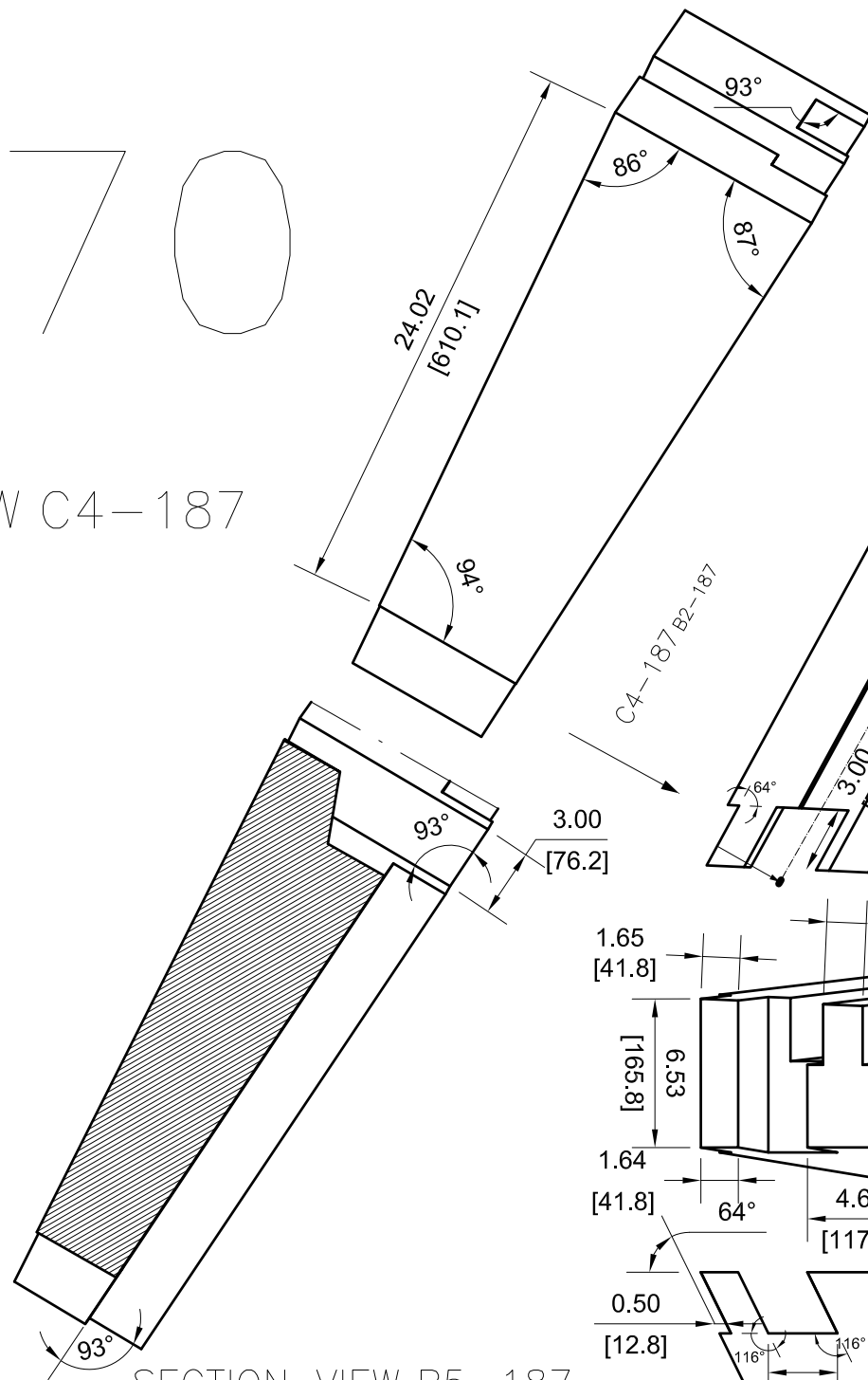
SECTION VIEW B5-187
