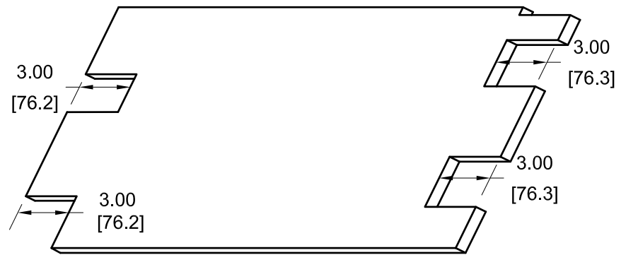
REAR VIEW RELATIVE TO VIEW E4-183
