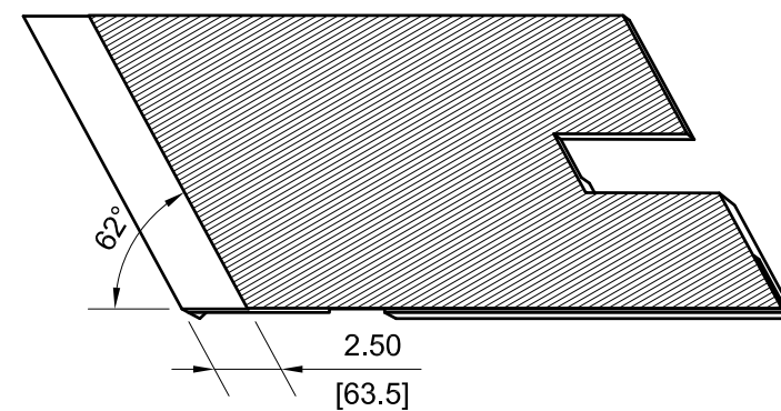
SECTION VIEW F6-80
