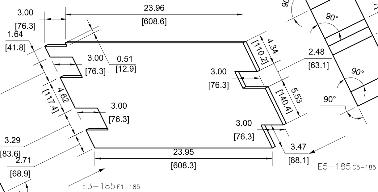
REAR VIEW RELATIVE TO VIEW D4-185
