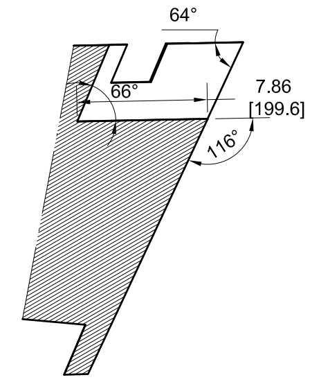
SECTION VIEW A5-132
