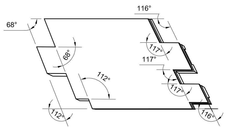
VIEW D4-137 REPEATED FOR CLARITY PURPOSES.
