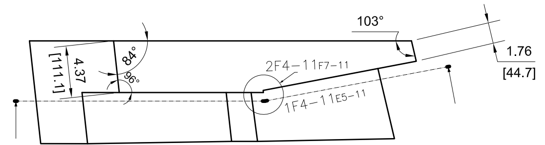
SECTION VIEW 1F4-11
