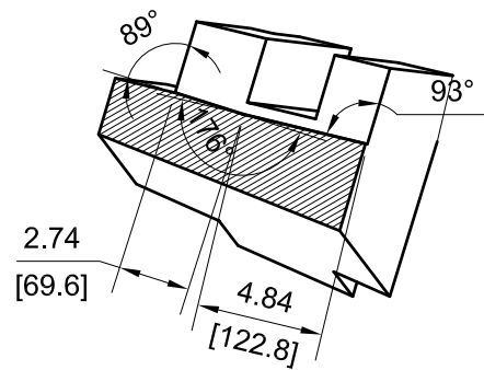
SECTION VIEW D3-90
