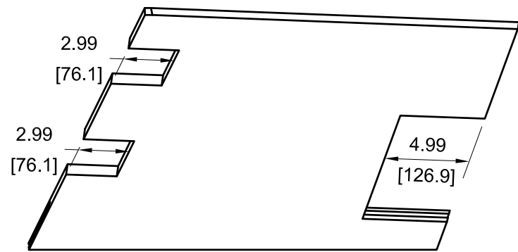
REAR VIEW RELATIVE TO VIEW D4-134
