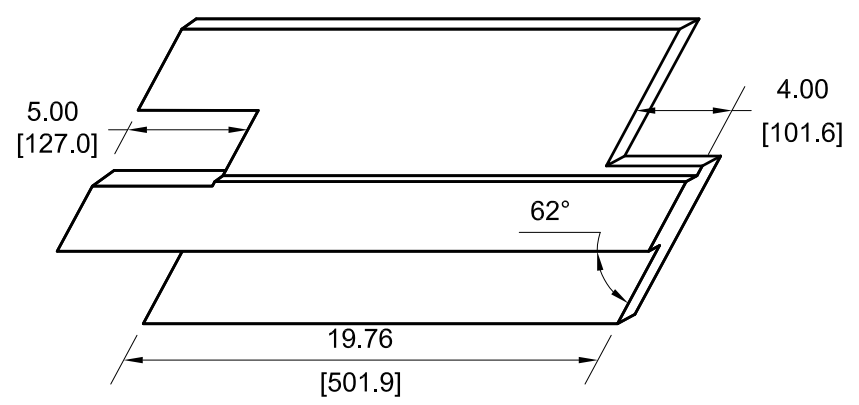
REAR VIEW RELATIVE TO VIEW D4-96
