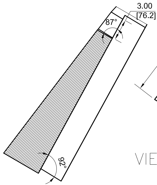
SECTION VIEW B5-157
