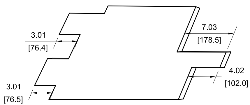
REAR VIEW RELATIVE TO VIEW D4-144
