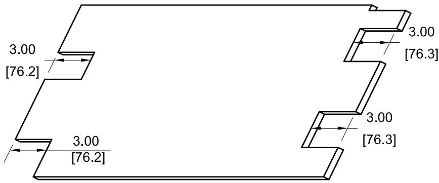
REAR VIEW RELATIVE TO VIEW D4-185
