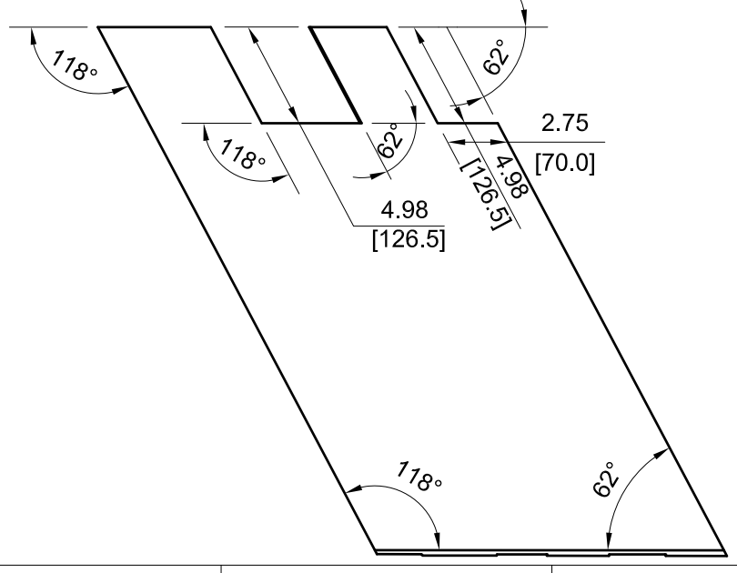
VIEW D4-125 REPEATED FOR CLARITY PURPOSES.
