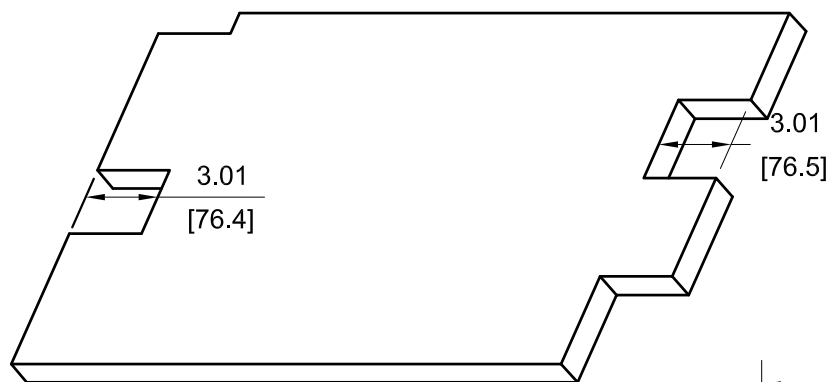
REAR VIEW RELATIVE TO VIEW D4-174
