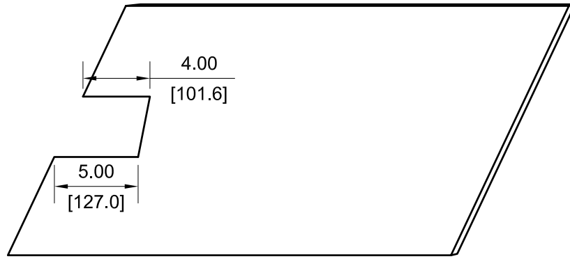
REAR VIEW RELATIVE TO VIEW D4-10
