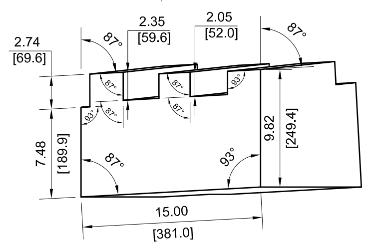
VIEW C4-56 A4-56
