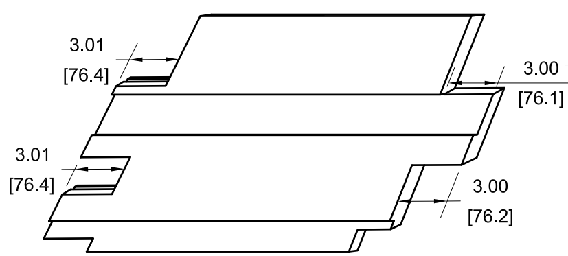
REAR VIEW RELATIVE TO VIEW C4-137
