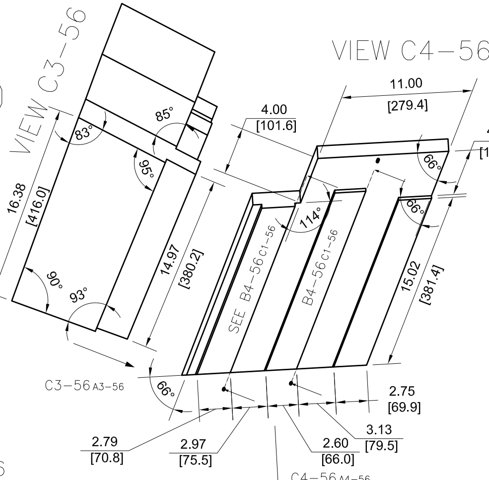
VIEW C4-56 A4-56
