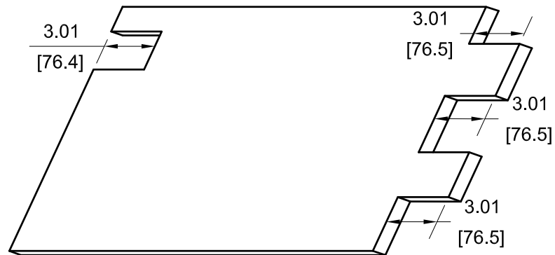
REAR VIEW RELATIVE TO VIEW D4-161
