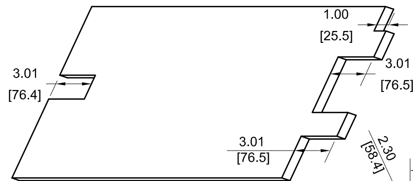
REAR VIEW RELATIVE TO VIEW D4-167
