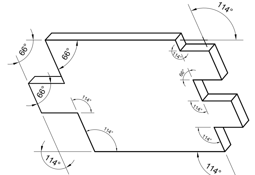
VIEW D4-178 REPEATED FOR CLARITY PURPOSES.
