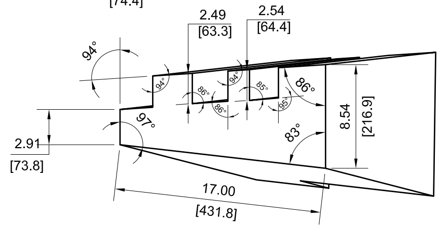
REAR VIEW RELATIVE TO VIEW D4-95
