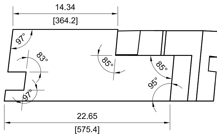
REAR VIEW RELATIVE TO VIEW D4-80
