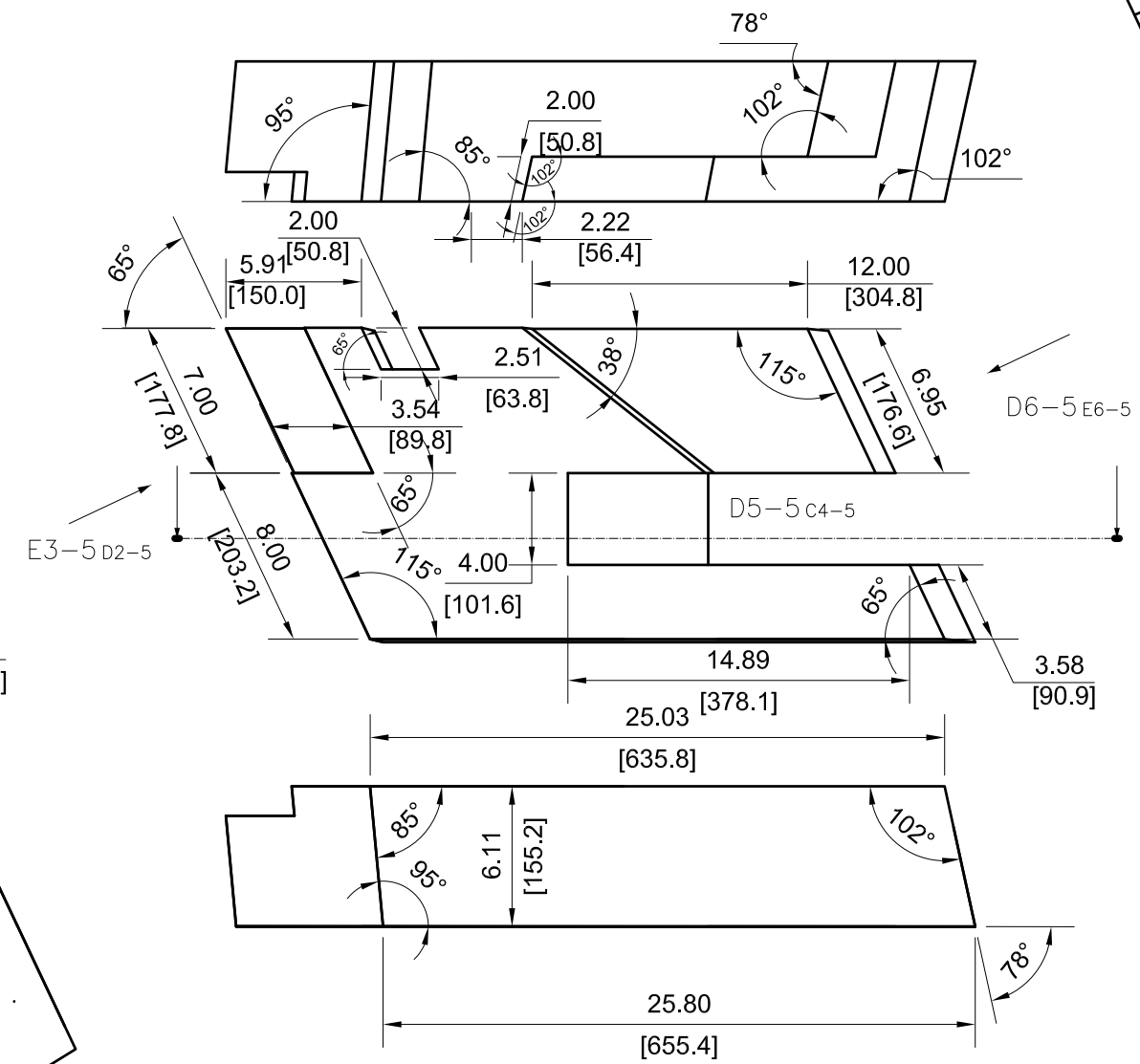
SECTION VIEW E2-5
