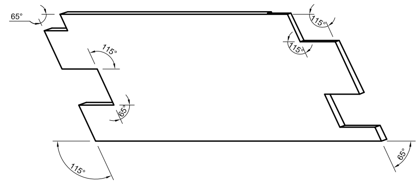
VIEW D4-153 REPEATED FOR CLARITY PURPOSES.
