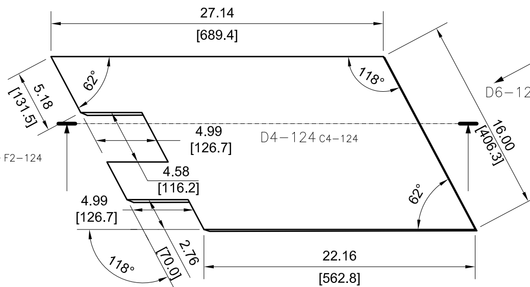
SECTION VIEW D4-124
