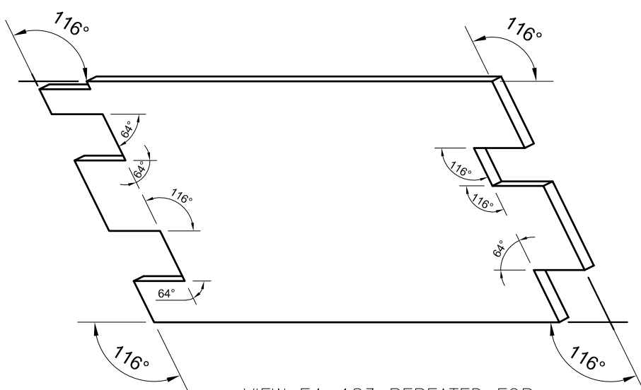
VIEW E4-183 REPEATED FOR CLARITY PURPOSES.
