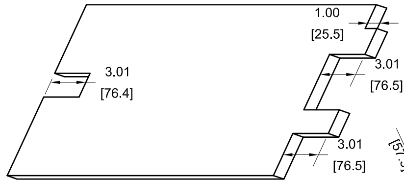
REAR VIEW RELATIVE TO VIEW D4-165
