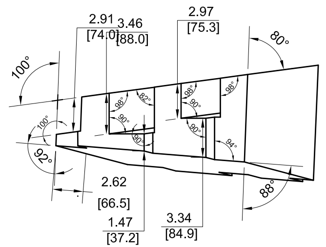
VIEW E4-141 REPEATED FOR CLARITY PURPOSES.
