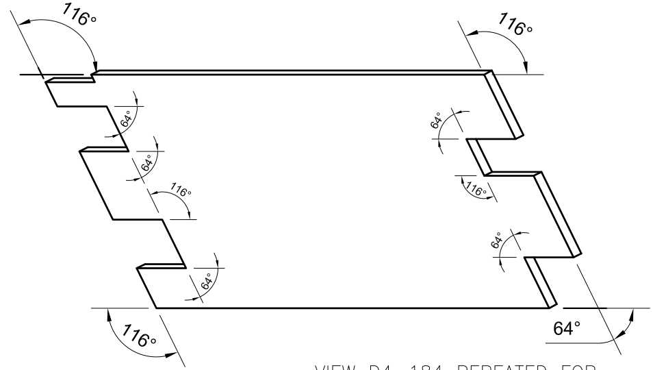
VIEW D4-184 REPEATED FOR CLARITY PURPOSES.
