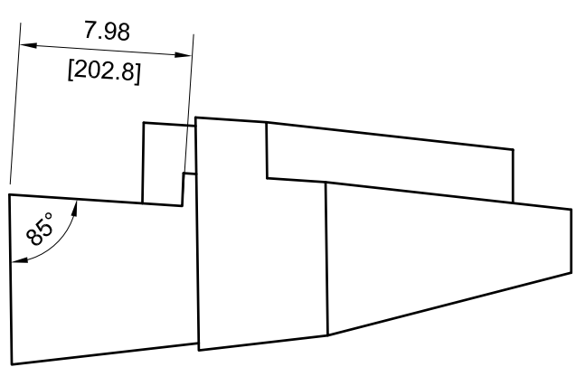
REAR VIEW RELATIVE TO VIEW D4-95
