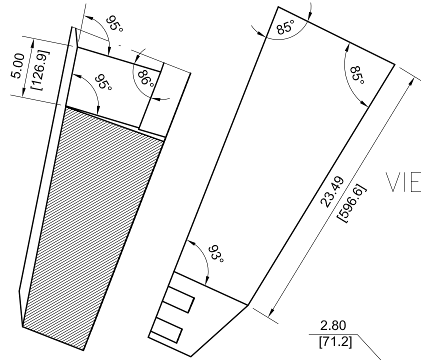
SECTION VIEW C3-84
