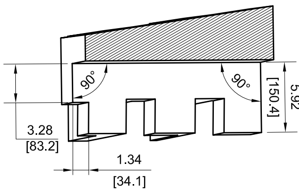
SECTION VIEW C5-131
