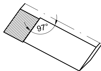
SECTION VIEW D3-68
