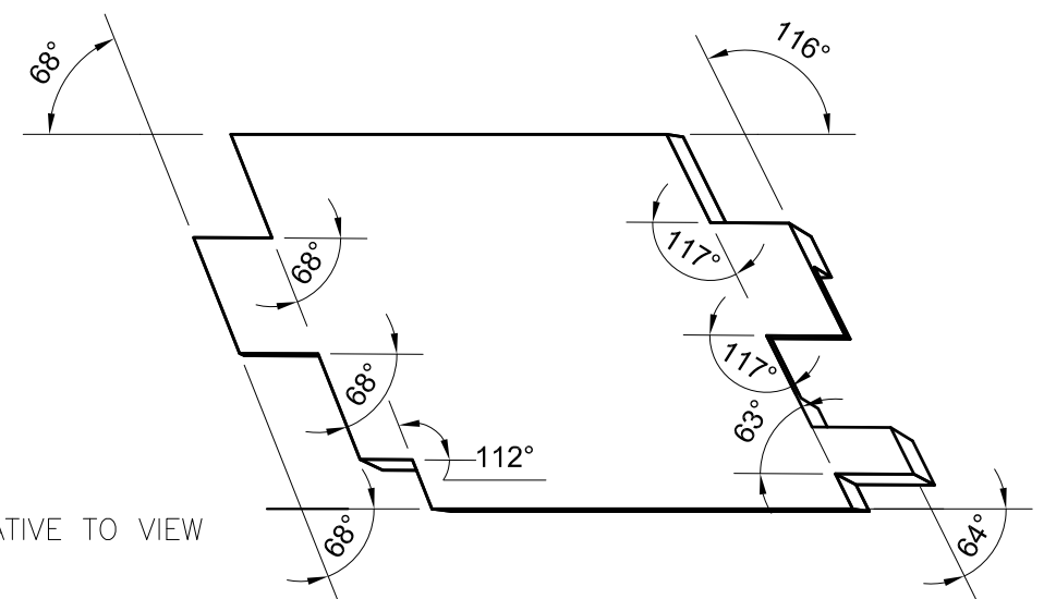
VIEW C4-138 REPEATED FOR CLARITY PURPOSES.
