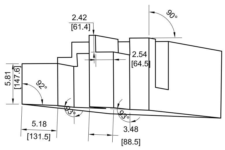
VIEW D4-125 REPEATED FOR CLARITY PURPOSES.
