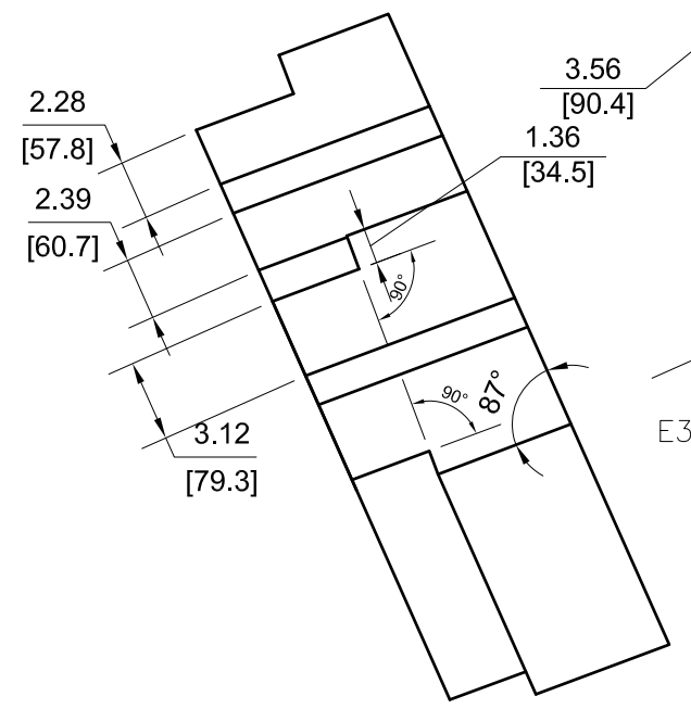
REAR VIEW RELATIVE TO VIEW D4-170
